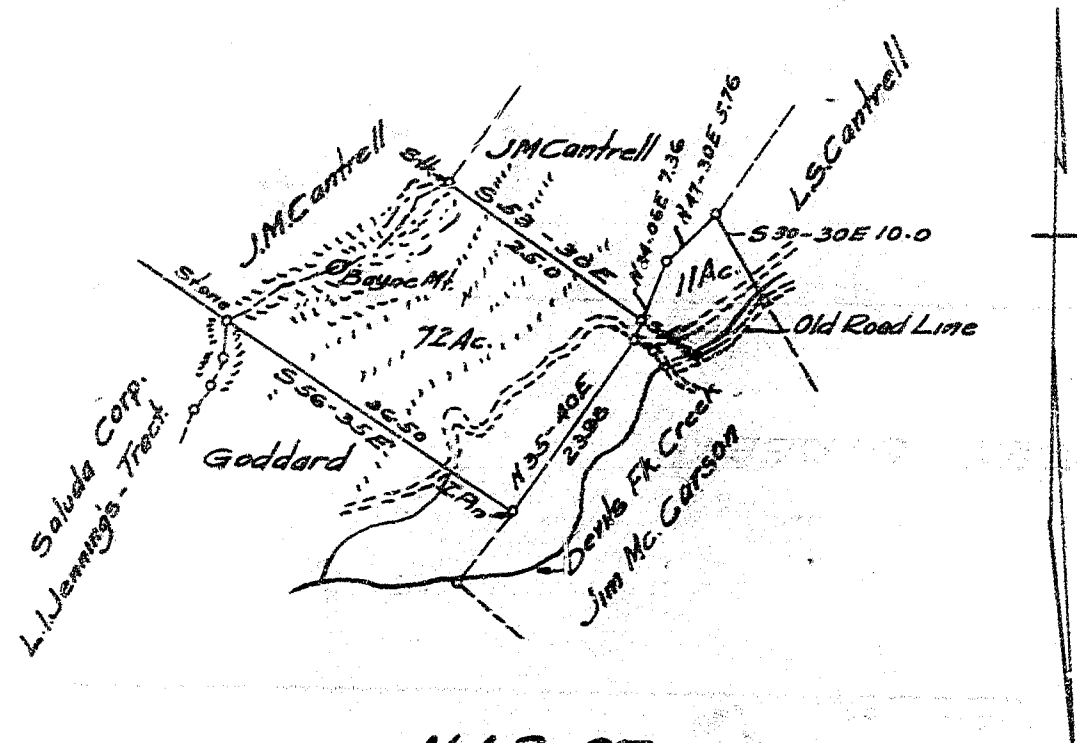
MAP OF L.S. CANTRELL LAND GREENVILLE, CO. SC. Scale 1" = 20 ch. SURVEYED 9/20 Rec. APR. 21. Howard Wiswall C.E.
